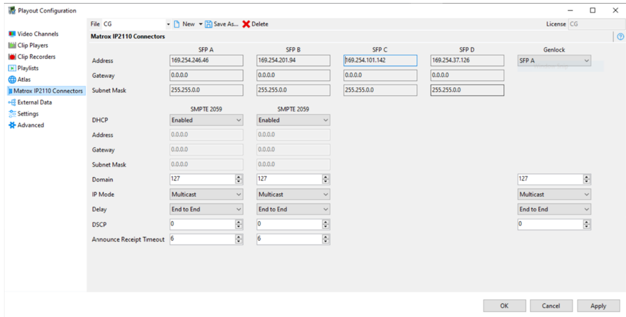
Genlock over IP Configuration with SMPTE 2059 for the DSXLE5 IP Q25
